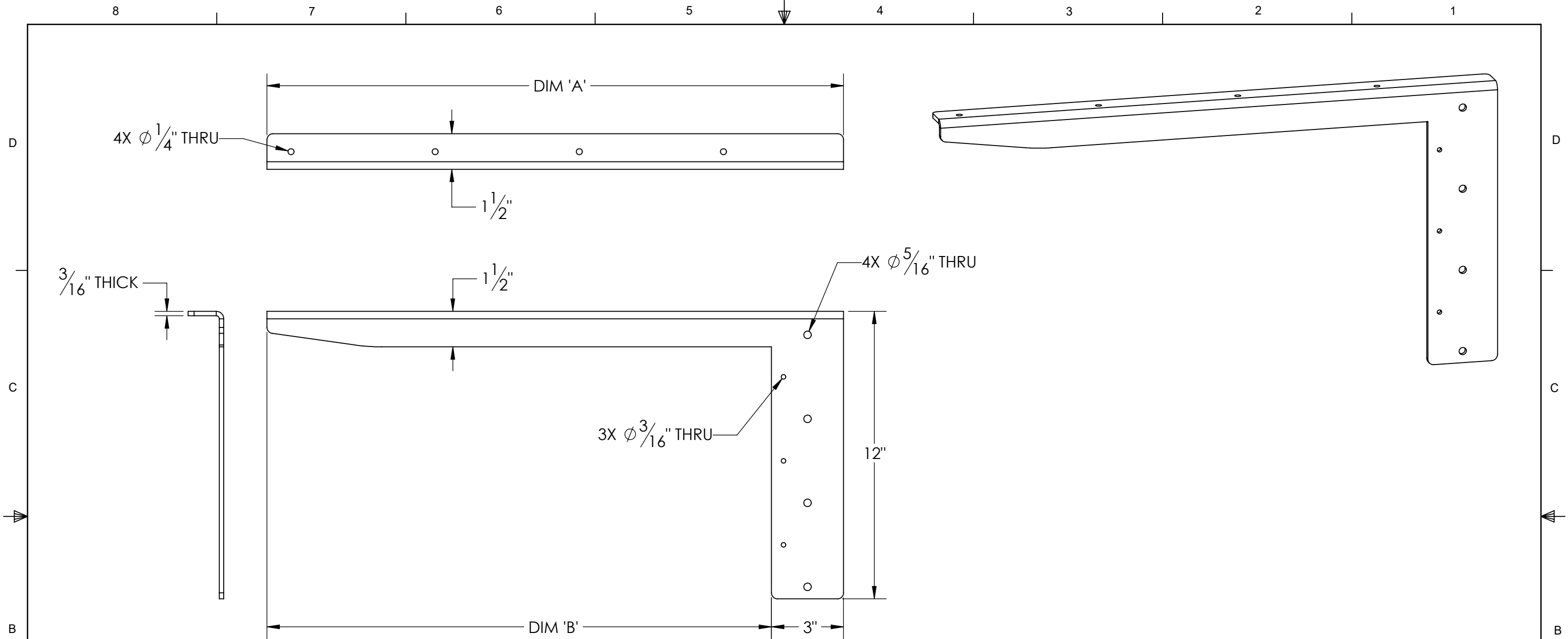
CT-BM-24-LT LEFTHAND VERSION SHOWN
